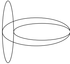
FIGURE 3. A triple of conics in (C3) configuration
