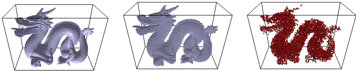
Figure 18: Left: Dragon with 500k faces. Middle: LDI representation with a resolution of 64x64. Right: Particles penetrating the volume of the dragon are detected. In this environment with 500k faces, 100k particles can be tested for penetration in 225 ms using a standard PC.
