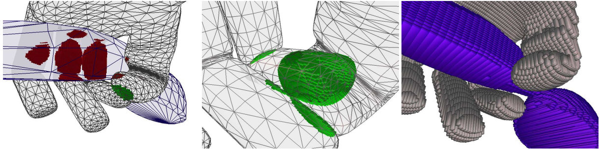
Figure 17: Left: Collisions (red) and self-collisions (green) of the hand are detected. Middle: Self-collisions (green) are detected. Right: LDI representation with a resolution of 64x64. Collisions and self-collisions are detected in 8-11 ms using a standard PC.
