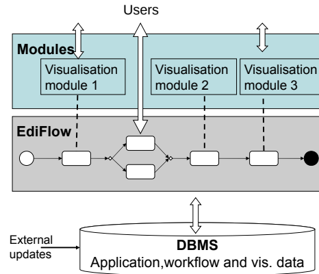
Figure 4: EdiFlow architecture.
