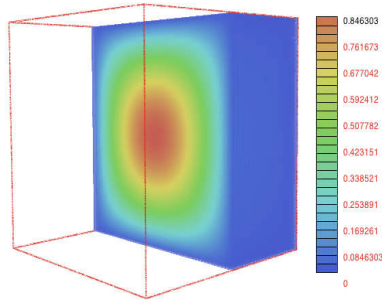
(a) initial control lattice
