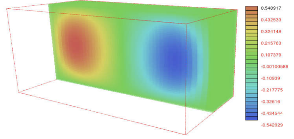
(b) initial solution field
