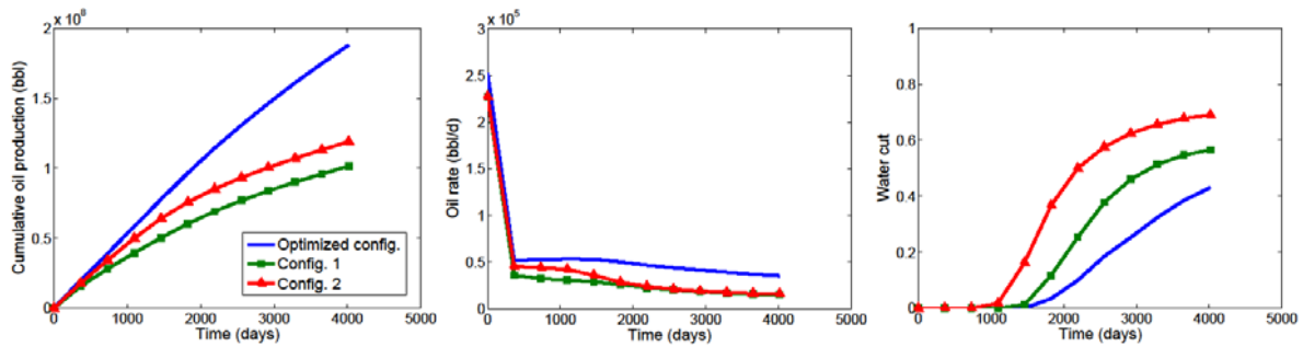
Fig. 10: Production curves for an optimized solution using CMA-ES with meta-models ( optimized config. ) and 2 engineer's proposed configurations ( config.1 and config.2 ).
