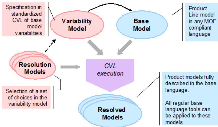
Figure 7 – Common Variability Language Approach
