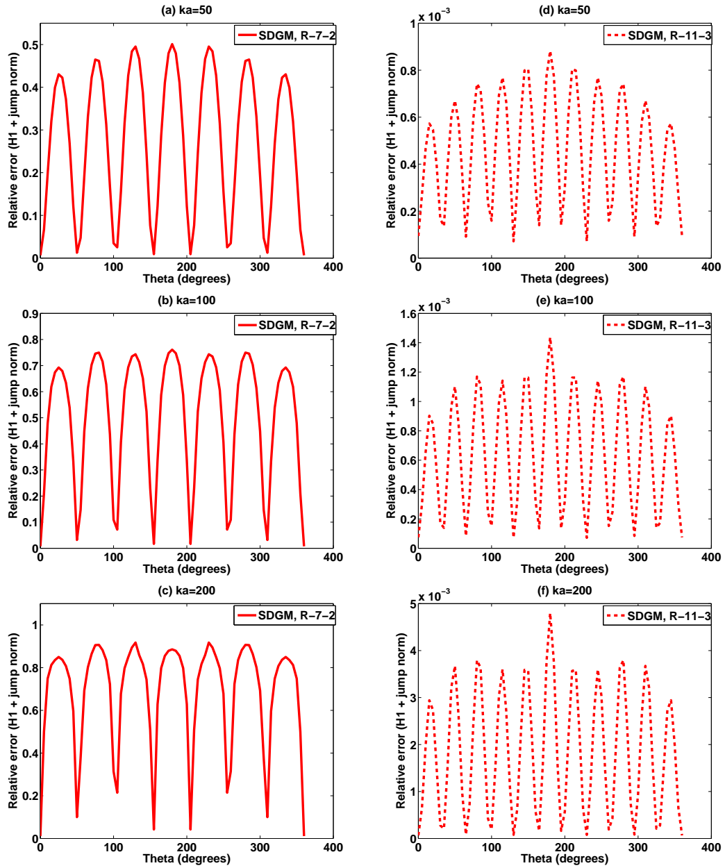
Figure 7: Performance comparison between SDGM equipped with R-7-2 (left) and R-11-3 (right), for a fixed resolution kh = 2 .
