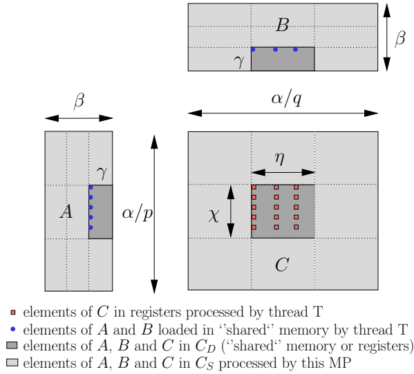
Figure 9: Tiling of matrices within a multi-processor
