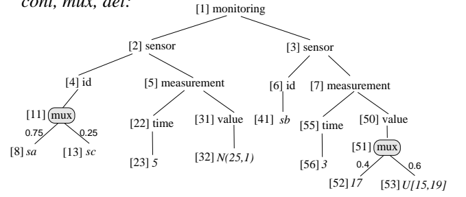
Figure 6: \text{PrXML}^{\text{cont}, \text{mux}, \text{det}} p-document: monitoring.
