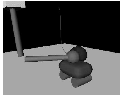
Figure 7: A three links articulated arm has to kick down a ball lying on a moving wagon. The desired final trajectory for the hand (position to reach and tangent to the spline curve) are defined in local coordinates relative to the ball. The contact between the ball and the wagon and the collision with the hand are automatically detected and treated by the simulation.
