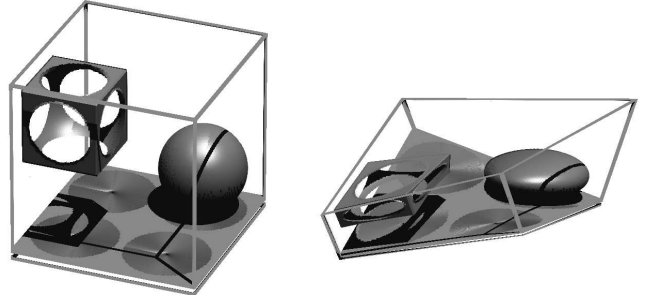
Fig. 11. The deformation affects not only the shape but also the reflective properties. The illumination is not simply deformed as if it was painted onto the surfaces, because the normals transformation is not the same as the points transformation.
