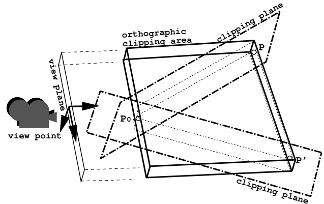
Figure 5. Naive approach using an orthographic camera.
