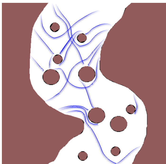
Fig. 11. Shockwaves built upstream and downstream obstacles.
