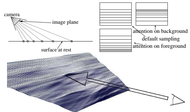
Figure 1: Dynamically adapted surface mesh, whose elements approximately have the same projected area on screen.
