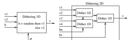
Figure 8: The dithering operators.
