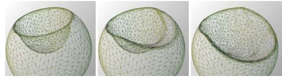
Figure 38: Behaviour of our mesh-updating algorithm on an already punched sphere. The decimation accompanying the second punch simplifies the small triangle of the first punch. The tool has been removed for better visualization.
