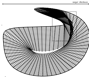
Figure 31: Folding for extreme shell thickness (prescribed thickness equal to the objects bounding box size, only 70% of the shell is shown to show the fold clearly.)
