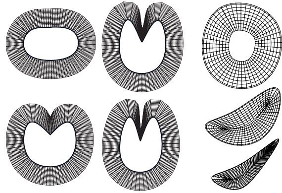
Figure 28: The four diagrams on the left show self-adjusting shell behavior of an exterior shell in the concave region. With an angle of up to 90 degrees, no compression in shell thickness is observed, but at greater angles the shell starts to compress. The three diagrams in the right column illustrate an interior shell. The first image shows the interior shell for which a prescribed thickness is achieved. As the object is deformed, the shell compresses to avoid folds (prescribed thickness remains the same).
