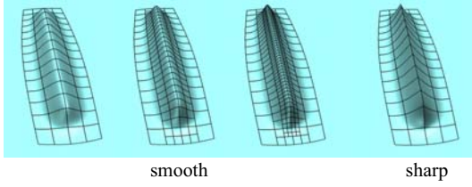
Figure 17: Multiresolution details are required to approximate sharp features using smooth surface representations (left three images). A piecewise smooth surface representation (right) allows sharp features to be modeled with detail vectors.
