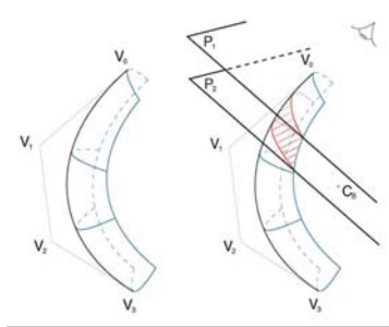
Figure 2: Left: Infering a local surface from a 2D stroke. Right: Rendering a slice of this model to create a new silhouette from another viewpoint.
