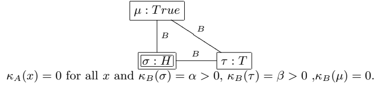
Fig. 7. be-action-model for the action ‘A cheats’
