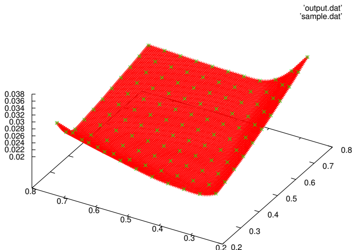
Figure 5: Drag coefficient in the design space
