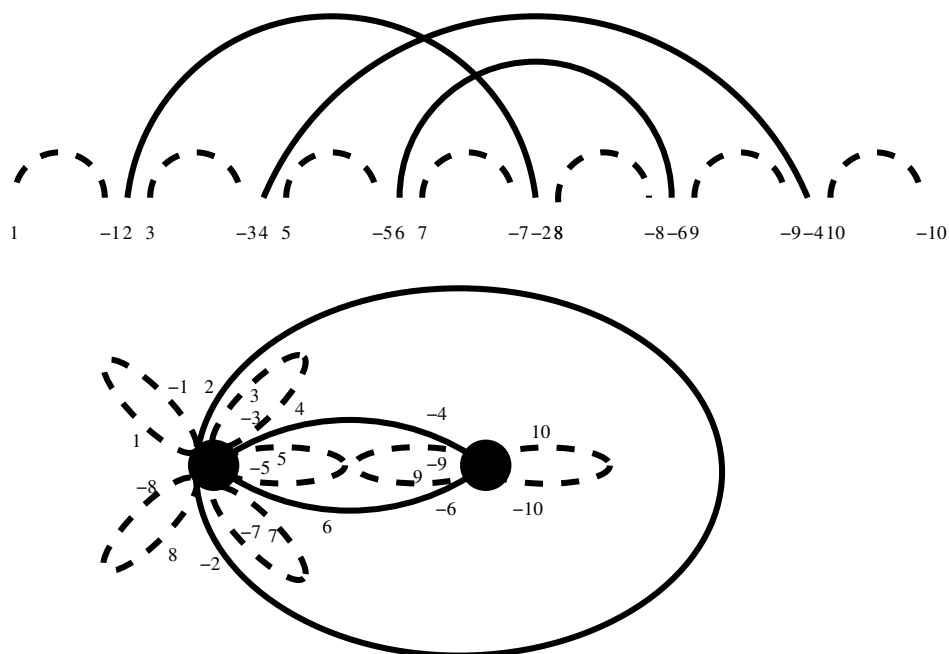
Figure 6: Top, a L&P structure corresponding to case 2. Bottom, the corresponding planar map. Arcs not involved in the pseudoknot are drawn in dotted lines.
