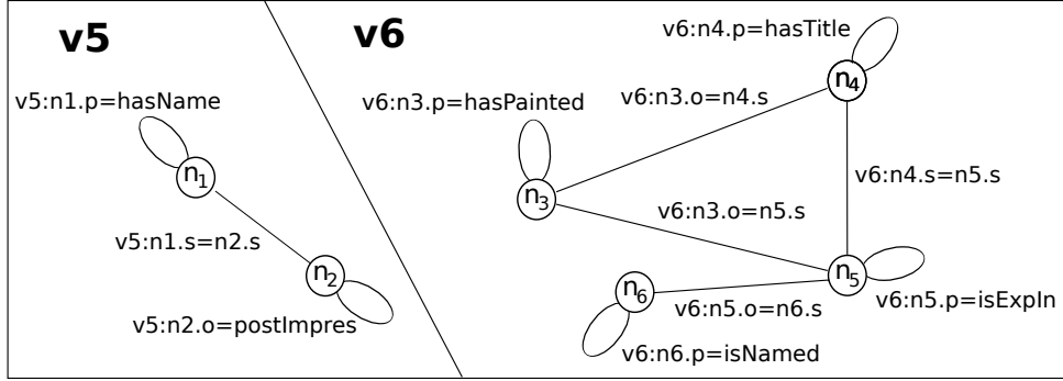
Figure 3: State graph after two join cuts.
