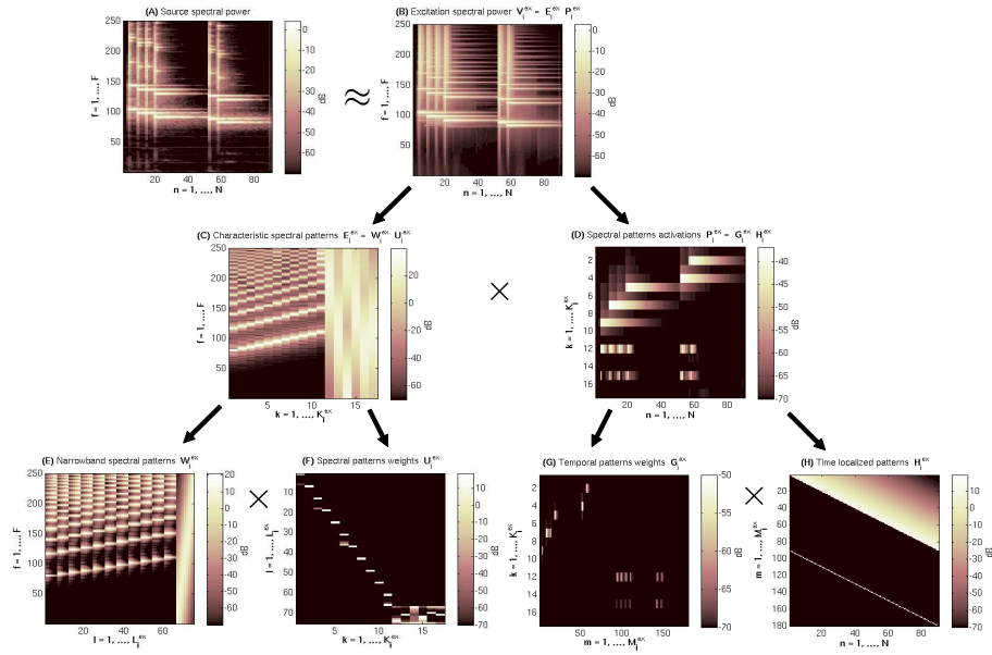
Figure 3: Excitation power decomposition V_j^{\text{ex}} = W_j^{\text{ex}} U_j^{\text{ex}} G_j^{\text{ex}} H_j^{\text{ex}} as applied to the spectral power of several xylophone notes. (A): source spectral power, (B): excitation spectral power V_j^{\text{ex}} = E_j^{\text{ex}} P_j^{\text{ex}} , (C): characteristic spectral patterns E_j^{\text{ex}} = W_j^{\text{ex}} U_j^{\text{ex}} , (D): spectral pattern activations P_j^{\text{ex}} = G_j^{\text{ex}} H_j^{\text{ex}} , (E): narrowband spectral patterns W_j^{\text{ex}} , (F): spectral pattern weights U_j^{\text{ex}} , (G): temporal pattern weights G_j^{\text{ex}} , (H): time-localized patterns H_j^{\text{ex}} .
