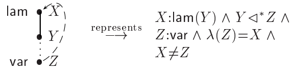
Figure 2. A constraint graph representing an overlap-free constraint.
