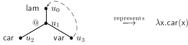
Figure 1. A \lambda -structure and the \lambda -term it represents.
