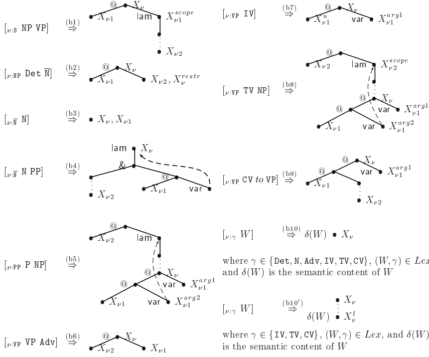
Figure 12. The syntax/semantics interface
