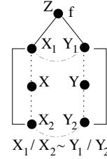
Fig. 10. Correspondence
