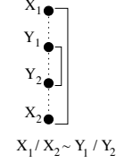
Fig.21. Termination?
