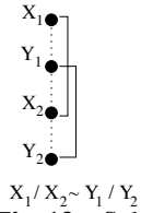
Fig. 13. Self-overlap
