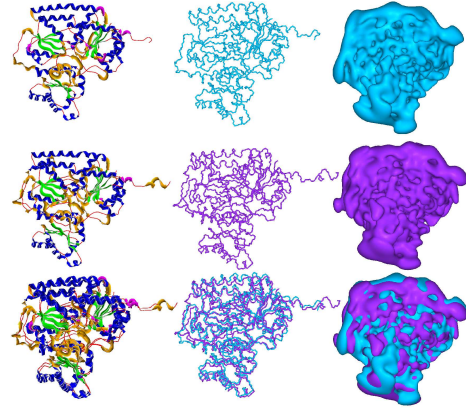
Figure 2: The superposition of a pair of nitrogenase proteins, shown as ribbon cartoons (left), backbone traces (middle), and as 3D SPF density expansions to order N=25 (right). The protein in the top row is from azotobacter vinlandii (PDB code 2MIN). Top row: PDB code 2MIN; middle row PDB code 1MIO; bottom row their superposed orientation. The two proteins have a sequence identity of 43%.
