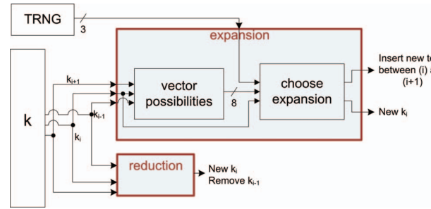
Fig. 4. Architecture of on-the-fly recoding unit with random DBNS representations.
