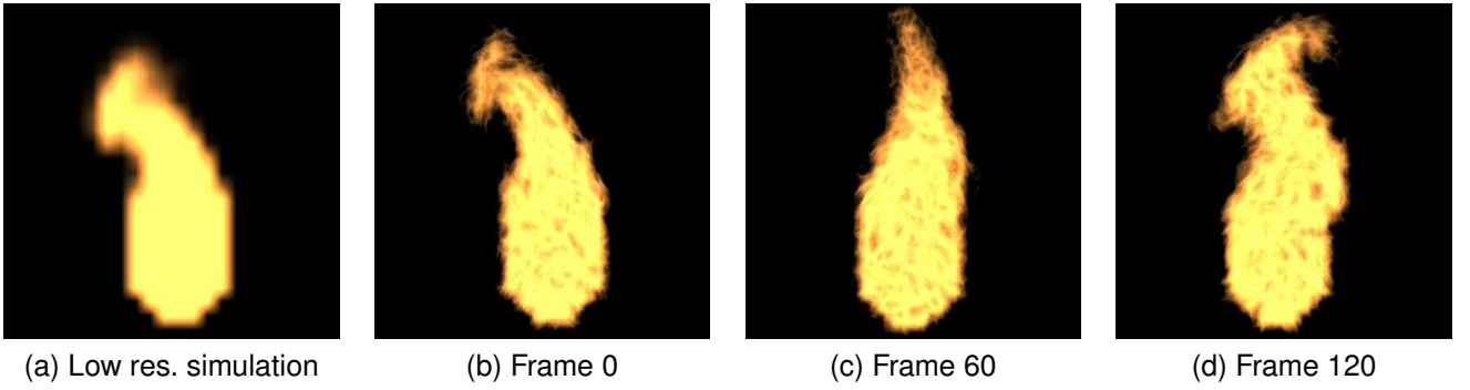
Fig. 4. Using a Perlin noise reference texture advected by our method to add details at (512 \times 512) resolution to a low resolution 2D fire simulation ( 32 \times 32 velocity and marker density fields, cf (a)). Here, the reference texture is analytic (no storage): 4 bands of time varying noise are used, a_j(\mathbf{x}) = b_j(2^j \mathbf{x}, t) and F(\{a_j\}) = LUT(dens(\mathbf{x}, t) + scale \sum \frac{1}{2^j} (1 - |2a_j - 1|)) . See also the accompanying video.
