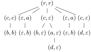
Figure 5: An editing script from the XQUF query of figure 1.
