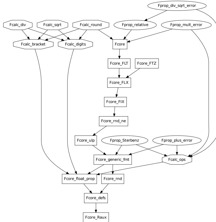
Fig. 2. Dependency graph of the library. Theorems from one file depend on the theorems from the pointed files. The shapes of the node classify the origin of the files: rectangles for the core library (Section III), octagons for the computable operators (Section IV-A), and ellipses for the high-level properties (Section IV-B).
