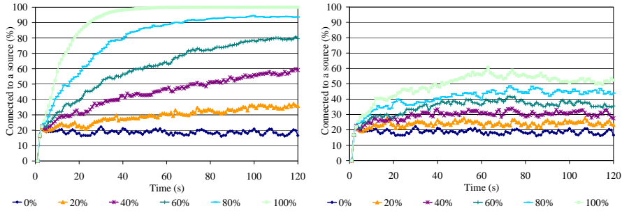
Fig. 10. Percentage of nodes stopping when connected, remaining nodes move randomly Fig. 11. Percentage of nodes that divide their speed by 6 when connected, remaining nodes move randomly
