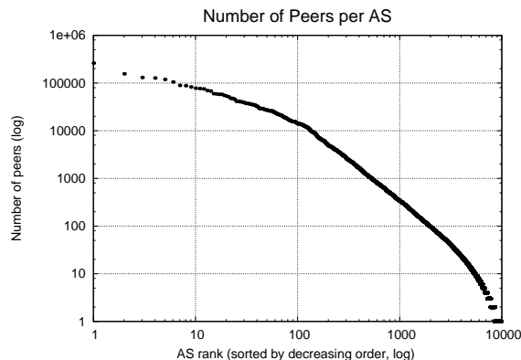
Figure 7: Distribution of the number of peers per AS. Most ASes have few peers.
