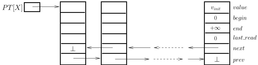
Figure 3: List implementing a transaction-level shared object X
