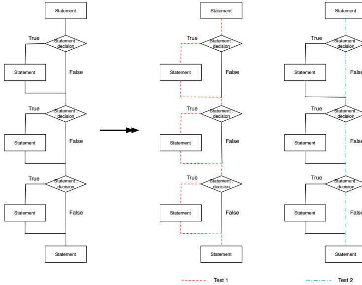
Figure 3.2: Paths considered by Branch Coverage at 100%.
