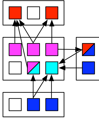
Figure 3.7: This figure illustrates some primitive metrics for packages. With respect to the central package: NCP(\text{Number of classes in package}) = 6 ; HC(\text{Hidden classes}) = 1 ; OutC(\text{package provider classes}) = 4 (magenta); InC(\text{Package used classes}) = 2 (cyan); SPC(\text{System provider classes}) = 3 (red); SCC(\text{System client classes}) = 4 (blue).
