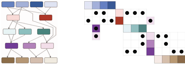
Fig. 3. A node-link depiction of a small layered graph (left) and its quilt depiction (right) [38].
