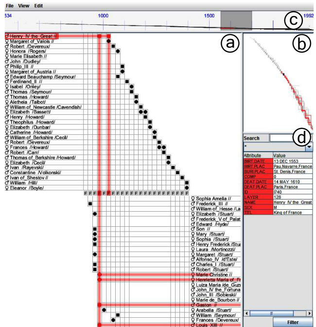
Fig. 4. The GeneaQuilts System showing part of the European Royal families. It consists of (a) the main visualization, (b) an overview, (c) a timeline and (d) a query and details panel.
