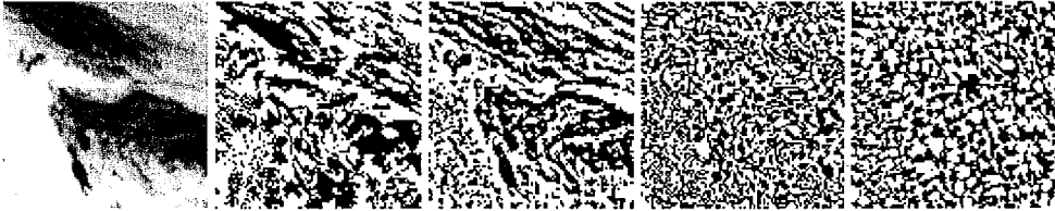
Figure 8: From left to right: spatial slice of an infrared image at noon, t = 12 h , its temporal and spatial edges coinciding with the interfaces and regions where \sigma_{edge}^t and \sigma_{edge}^s change or have a particular sign, the ridges, ruts and inflection lines coinciding with the interfaces where \sigma_{phase} changes sign, and the ridges occur where the signature of k_i is positive. The input image acquired between t = 9 h and t = 18 h consists of 18 temporal views of spatial slices composed of 200 \times 200 voxels each with a dynamic resolution of 8 bits .
