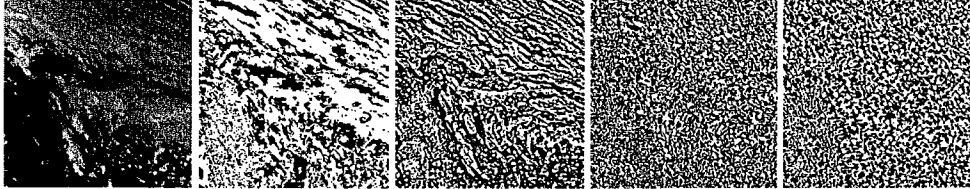
Figure 7: From left to right: spatial slice of an image in the visual spectrum at noon, t = 12 h , its temporal and spatial edges coinciding with the interfaces and regions where \sigma_{edge}^t and \sigma_{edge}^s change or have a particular sign, the ridges, ruts and inflection lines coinciding with the interfaces where \sigma_{phase} changes sign, and the ridges occur where the signature of k_i is positive. The input image acquired between t = 9 h and t = 18 h consists of 18 temporal views of spatial slices composed of 200 \times 200 voxels each with a dynamic resolution of 8 bits .
