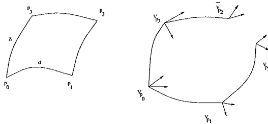
Figure 1: A closed circuit C = (p_0 p_1 p_2 p_3 p_0) on S and the frame field V along the upper part and lower part of circuit C .
