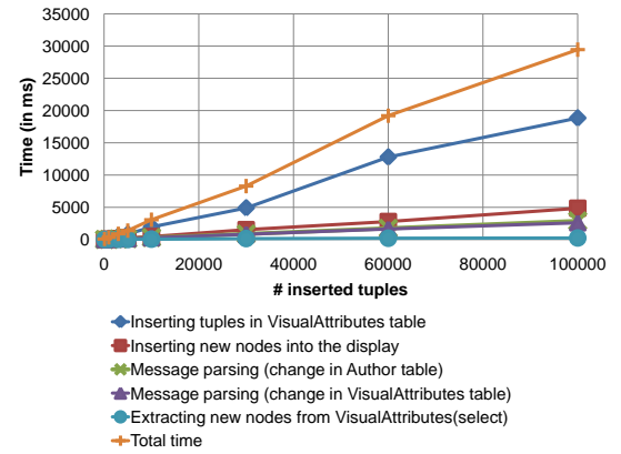
Fig. 8. Time to perform insert operation.
