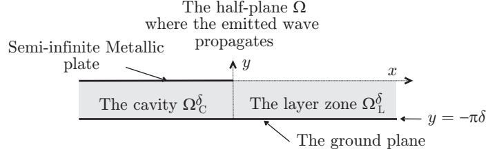
FIGURE 2. Two-dimensional geometry of the radiation problem
