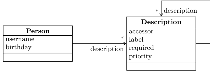
Fig. 3. The domain object Person with its Magritte meta-description.
