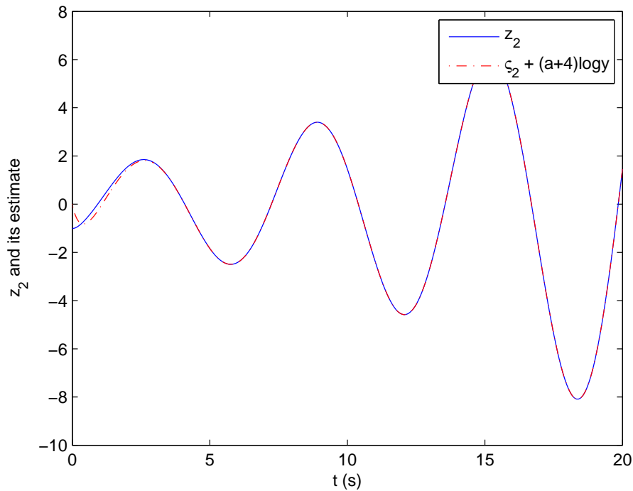
Fig. 5. z_2 and its estimate with initial conditions z_2(0) = -1 and \hat{z}_2(0) = \varsigma_2(0) = 0 .
