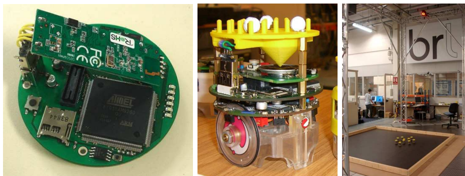
Figure 15. Left: e-puck Linux extension board with USB WiFi card (casing removed). Middle: An e-puck with Linux board fitted in between the e-puck motherboard (lower) and the e-puck speaker board (upper). Also note the yellow ‘hat’ which here serves three different functions: (1) it provides a matrix of pins for the reflective spheres which allow the tracking system to identify and track each robot, and (2) it provides a mounting for the USB WiFi card which slots in horizontally (the wires connecting to the WiFi card are above the USB connector). Right: experimental swarm robotics arena with 10 Linux extended e-pucks.
