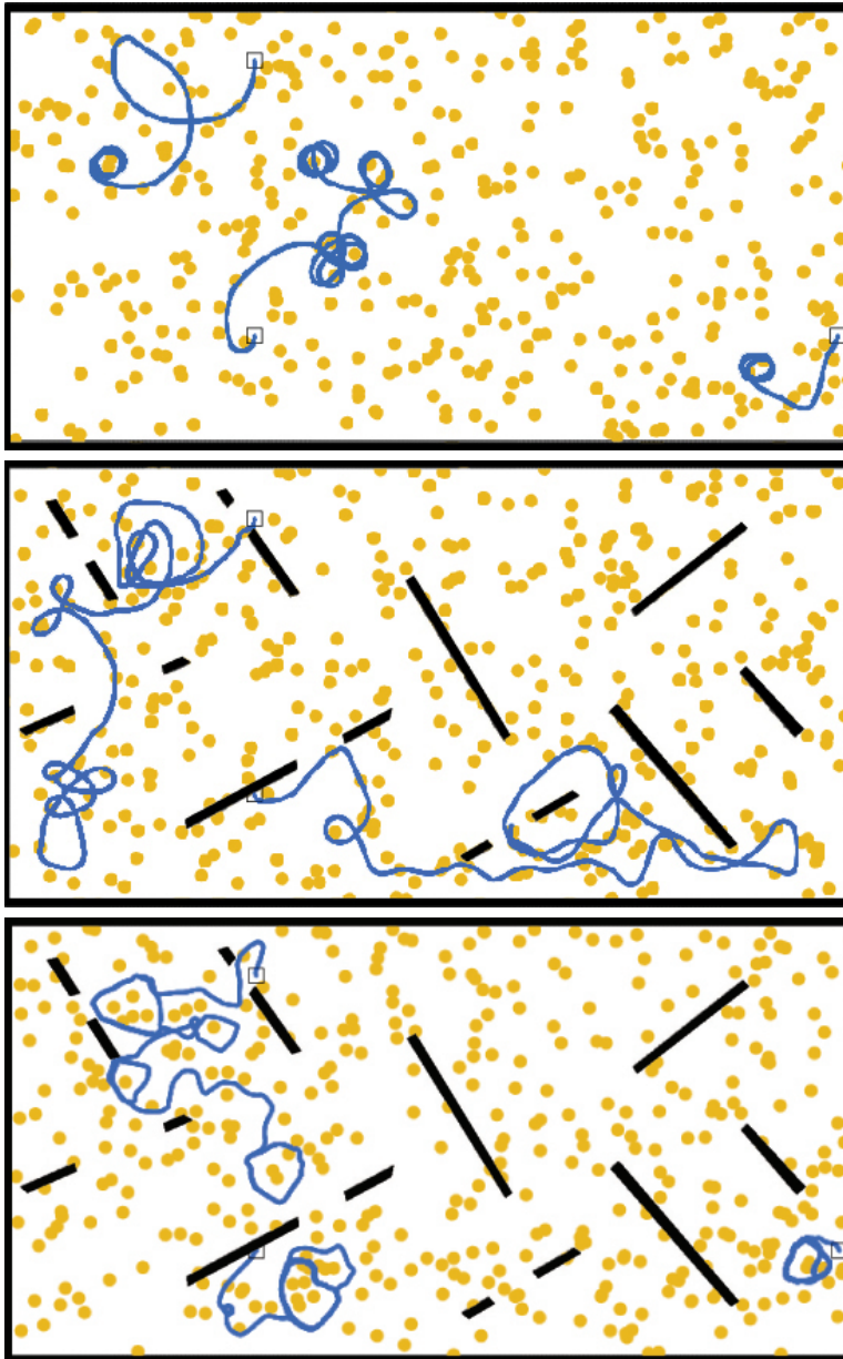
Figure 5. Typical examples of agents' behavioural traces in the free-ride setup. The square symbol shows the agent starting points. Agents are tested in environments with or without walls (i.e. black bars).
