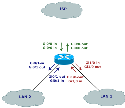
Fig. 4. ACLs Naming
