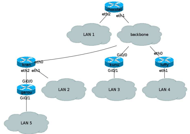
Fig. 5. Testbed - Initial network
