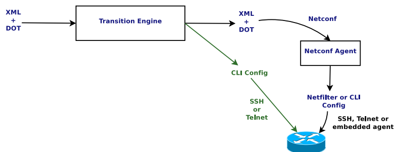
Figure 2.1: Planned Architecture
