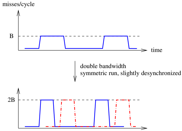
Figure 6: Example for explaining why self-performance can exceed the performance of an isolated run with memory bandwidth statically partitioned. This example assumes 2 cores.
