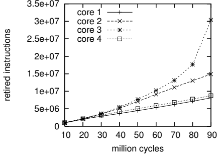
Figure 4: Symmetric run of microbenchmark 999 with SIZE = 2^{19} (Figure 3). Memory bandwidth is 4 bytes/cycle and the L2 replacement policy is a variant of DIP (one PSEL counter per thread). The plot shows the number of retired instructions on each core as a function of time.
