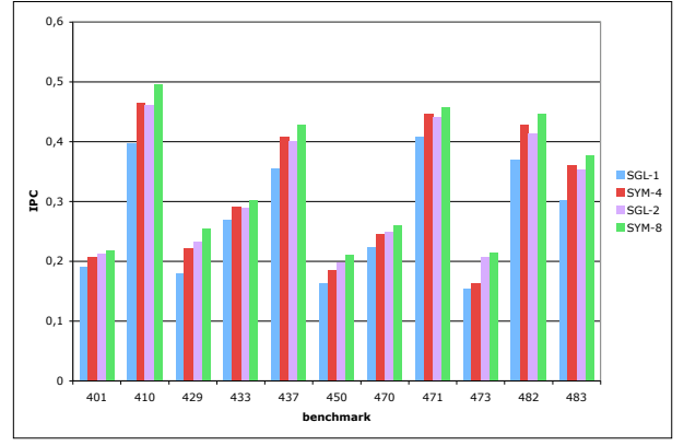
Figure 5: IPC per benchmark. Configuration SGL-1 is for an isolated run with a memory bandwidth of 1 byte per CPU cycle and a 1 MB shared cache. Configuration SYM-4 is for a symmetric run with a bandwidth of 4 bytes/cycle and a 4 MB cache. SGL-2 is for an isolated run with a bandwidth of 2 bytes/cycle and a 1 MB cache. SYM-8 is for a symmetric run with a bandwidth of 8 bytes/cycle and a 4 MB cache.
