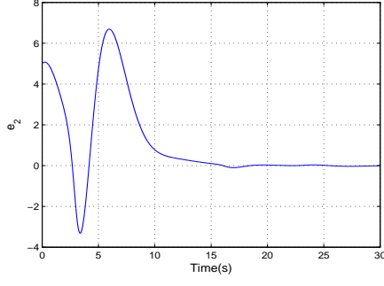
Fig. 6. Synchronization error on the state z_2
