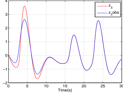
Fig. 7. z_3 and \hat{z}_3
