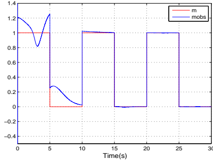
Fig. 13. Messages : m and \hat{m}
