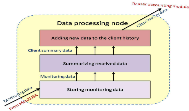
Figure 10: Architecture of a data processing node
