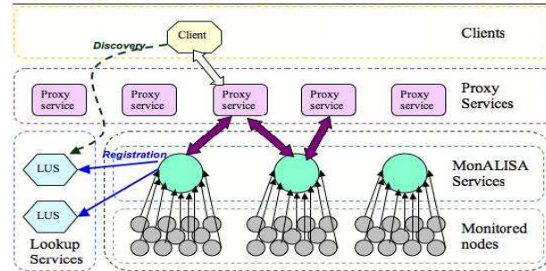
Figure 3: The MonALISA Architecture
