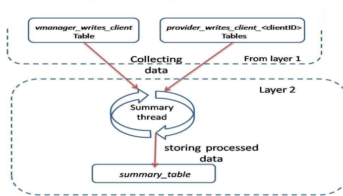
Figure 12: Data processing layer 2 - Creating a summary of the received data
