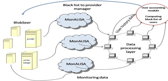
Figure 5: Distributed monitoring system infrastructure
