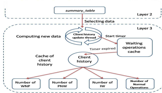
Figure 13: Data processing layer 3 - How the client history is being computed
