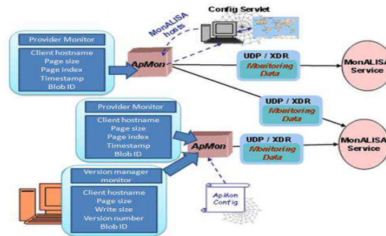
Figure 6: Collecting monitoring data from BlobSeer
