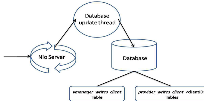
Figure 11: Data processing layer 1 - Storing data components
