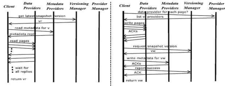
Figure 2: Internal interactions inside BlobSeer: READ(left) and WRITE(right)
