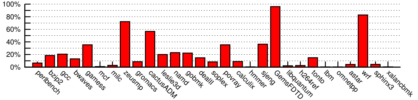
Figure 8: Dynamic null block access rate on main memory
