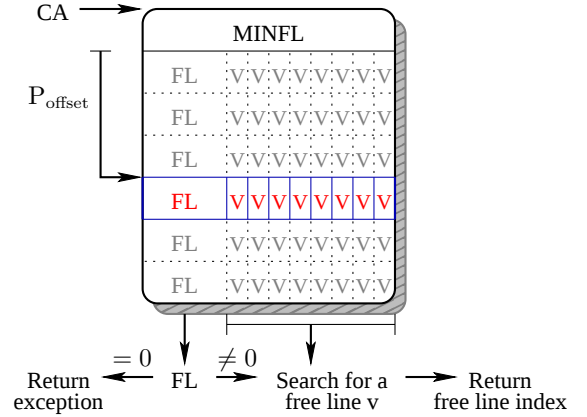
Figure 5: C-space descriptor and free line allocation.
