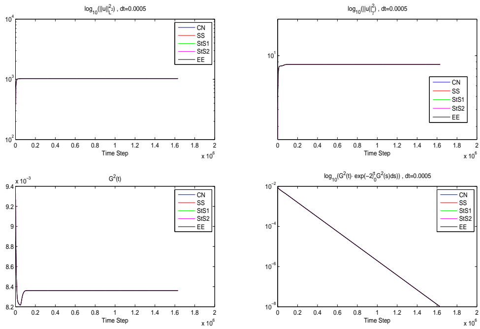
Figure 14: u_0(x) = S3, \gamma_k = \frac{1}{(1+|k|)^{1/4}}, f(x) = 0
