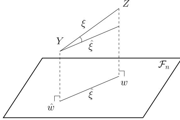
Figure 2: This figure shows the components used in Lemma 3 and its proof such as w , \hat{w} , \xi , and \hat{\xi} , and the fact that \langle \hat{\xi}, \xi \rangle_n = \|\hat{\xi}\|_n^2 .
