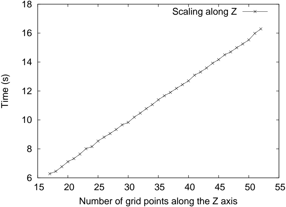
Figure 6. Strong scaling of the GPU three-dimensional finite-difference code running on a single GPU as a function of the number of points along Z , i.e., variation of the total time spent running the code on the GPU when the number of grid points along the Z axis of the grid increases. Scaling is almost linear, i.e., almost perfect.
