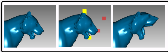
Fig. 1. Laplacian-based Deformation
