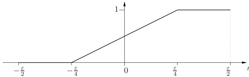
FIGURE 2. The extension function \chi_\varepsilon(s) .
